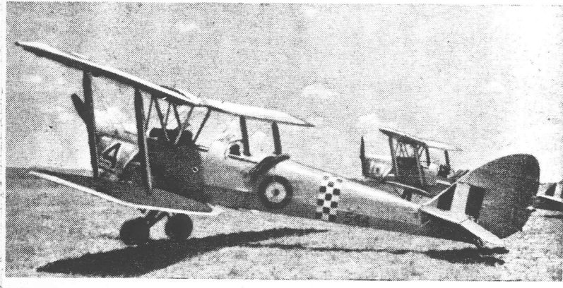
The Tiger Moth is one of several Australian-built examples. The machine shown was used at Mount Hampden and sported 56 Squadron "dicing."
