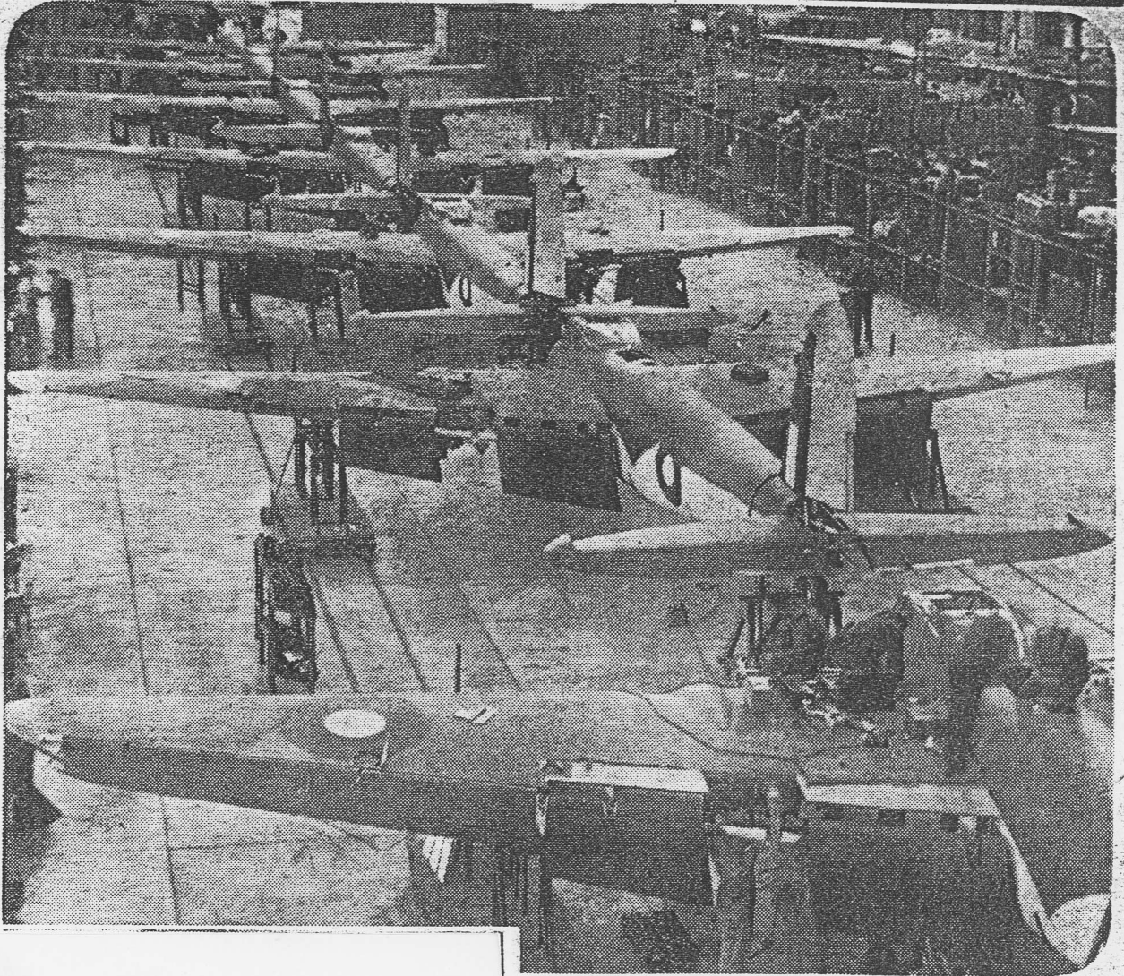
GENERAL VIEW OF THE N.S.W. FACTORY of the British company, De Havilland Aircraft Pty. Ltd., where Mosquito wood and metal fighter-bombers are now being built. First deliveries of these Australian-made aircraft have been made to the R.A.A.F. Left: A girl employee at the factory working on one of the Mosquitoes. She is employed as an electrical bonder.
