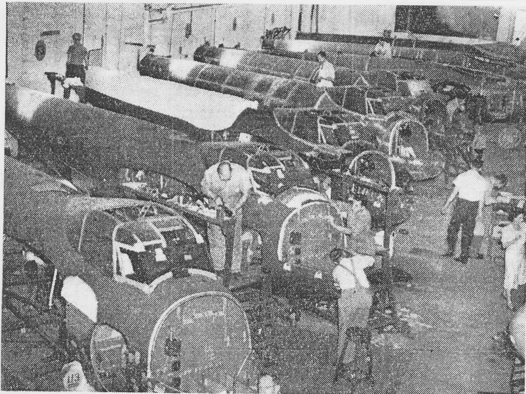
GENERAL VIEW OF THE N.S.W. FACTORY of the British company, De Havilland Aircraft Pty. Ltd., where Mosquito wood and metal fighter-bombers are now being built. First deliveries of these Australian-made aircraft have been made to the R.A.A.F. Left: A girl employee at the factory working on one of the Mosquitoes. She is employed as an electrical bonder.
