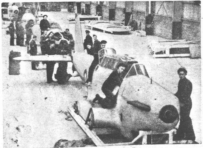
FAIREY BATTLE AIRCRAFT , a type new to Australia, are being assembled at an aircraft park in Victoria for training Empire Air Scheme recruits. Above: A view of the sleek tail of the training plane. Left: Fitters installing an engine. Below: A general view of the assembly line.
