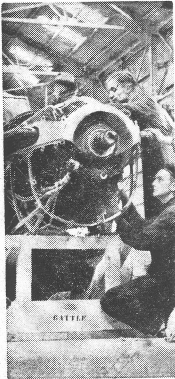
FAIREY BATTLE AIRCRAFT , a type new to Australia, are being assembled at an aircraft park in Victoria for training Empire Air Scheme recruits. Above: A view of the sleek tail of the training plane. Left: Fitters installing an engine. Below: A general view of the assembly line.
