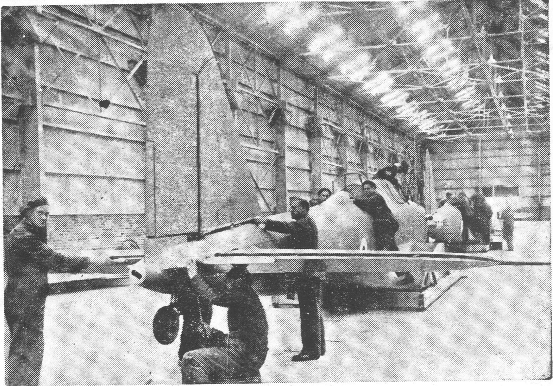
FAIREY BATTLE AIRCRAFT , a type new to Australia, are being assembled at an aircraft park in Victoria for training Empire Air Scheme recruits. Above: A view of the sleek tail of the training plane. Left: Fitters installing an engine. Below: A general view of the assembly line.
