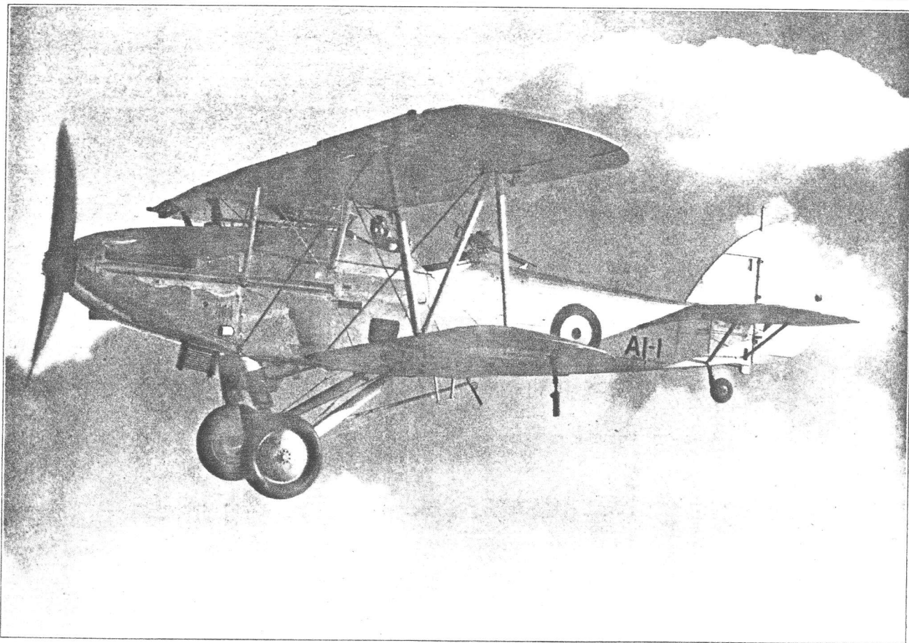
IMPERIAL DEFENCE.—A Hawker Demon (Rolls-Royce Kestrel) for the Australian Government. The hook for picking up messages and the tail-wheel are modifications from standard.
